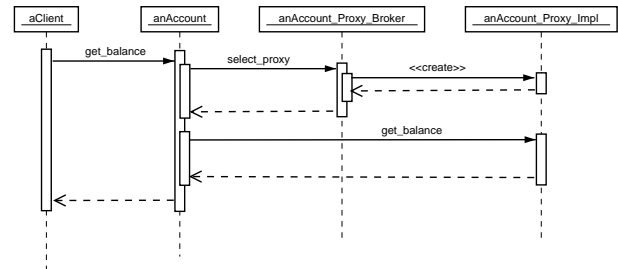
Figure 3: Interaction Diagram of the Virtual Component Pattern Applied in TAO
