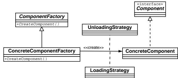
Figure 1: Virtual Component Static Structure.
