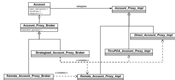
Figure 2: Static Structure of the Virtual Component Pattern Applied in TAO
