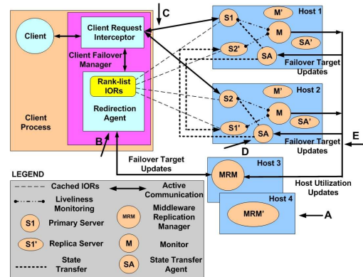
Figure 4: The FLARE Middleware Architecture
