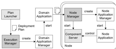
Figure 1: System Model for Component-based Deployment and Configuration
