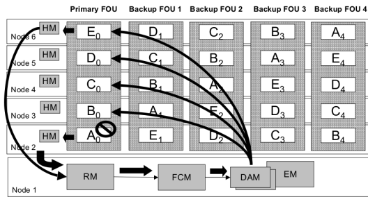
Figure 9: Experiment Setup for Failover Unit Shutdown Latency Measurement
