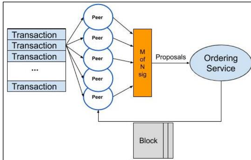
Fig. 8. Architecture of the PoA Consensus Mechanism in which nodes put their reputation at stake by verifying their identities before becoming miners in the network.
