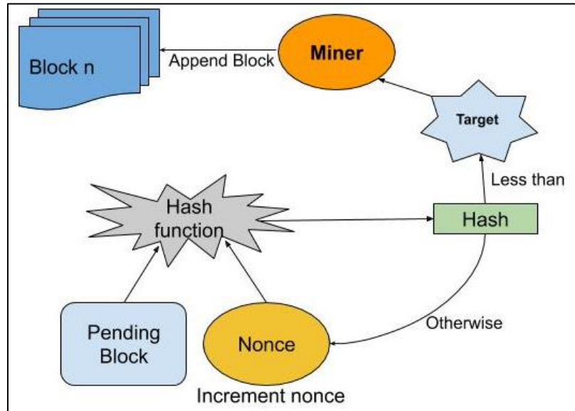
Fig. 2. The Iterative Process of Solving the Proof of Work Puzzle
