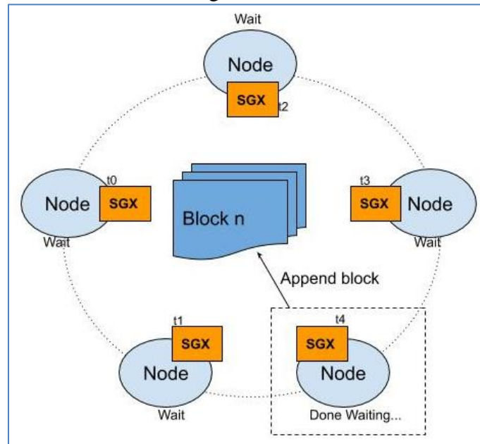
Fig. 6. Architecture of the PoET Consensus Mechanism that Leverages the Software Guard Extension (SGX) Technology to Select the Next Miner Based on A Random Wait Period.
