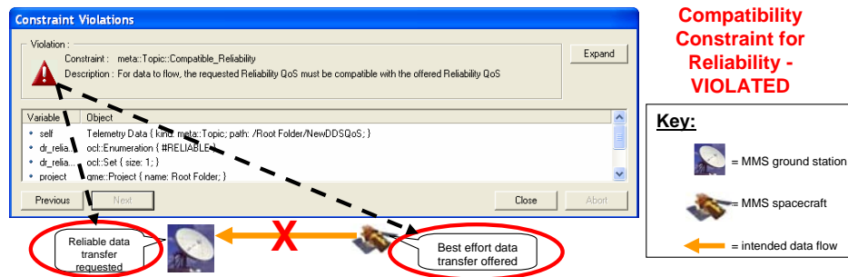
Fig. 8. Example of DQML QoS Policy Compatibility Constraint Checking
