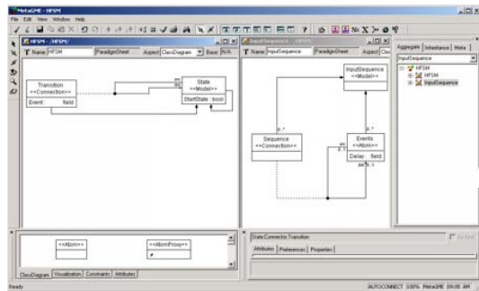
Source DSML Metamodel
