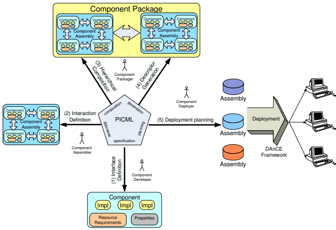
Fig. 1: Model-driven Application Development Lifecycle
