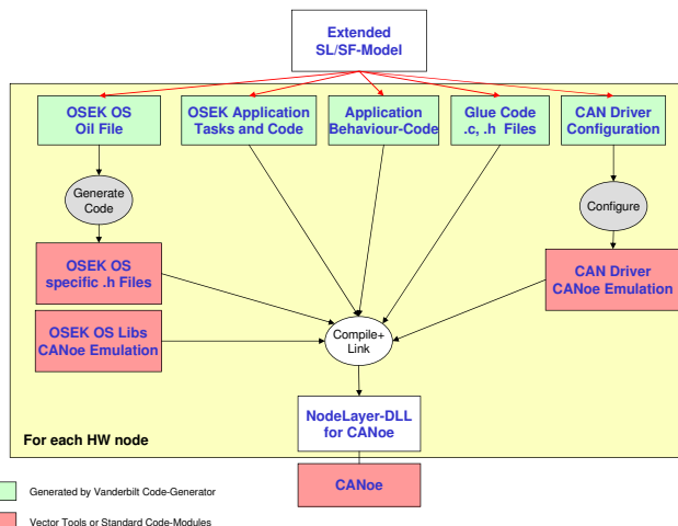
Fig. 3: ECSL Code Generation
