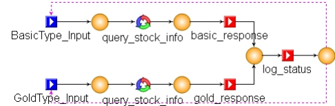
Fig. 6. Example CBML behavioral model with output actions.
