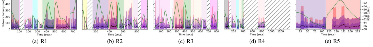
Fig. 7: Observed mean, std dev, 95 th and 99 th percentile network latencies and received signal strengths on emulated routes
