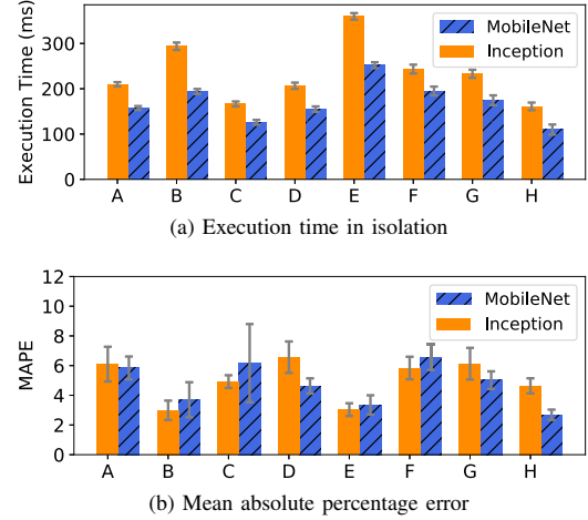
Fig. 5: Performance estimation model evaluations
