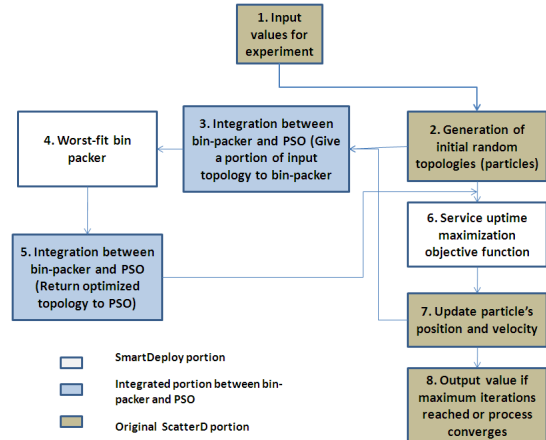
Fig. 2. SmartDeploy framework
