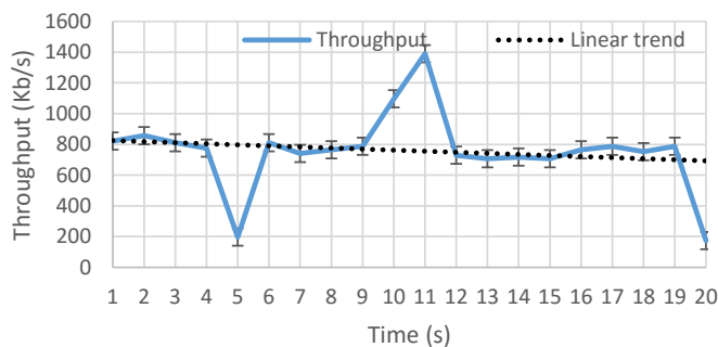
Fig. 5: Evaluating The Load Balancer with Traffic Redirection
