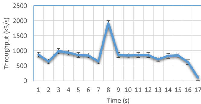
Fig. 7: Impact of the Packet Loss on The Bandwidth Fluctuation
