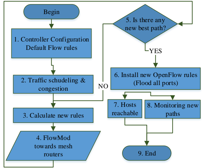
Fig. 4: The framework for the load balancer
