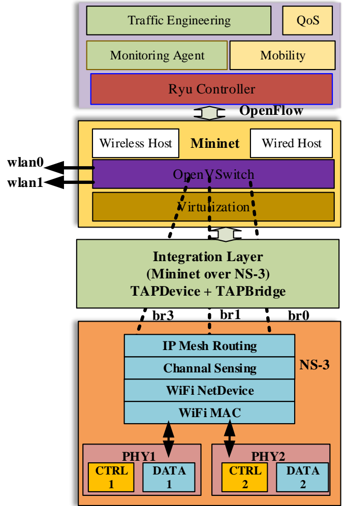
Fig. 2: Design of the OpenFlow-enabled mesh router
