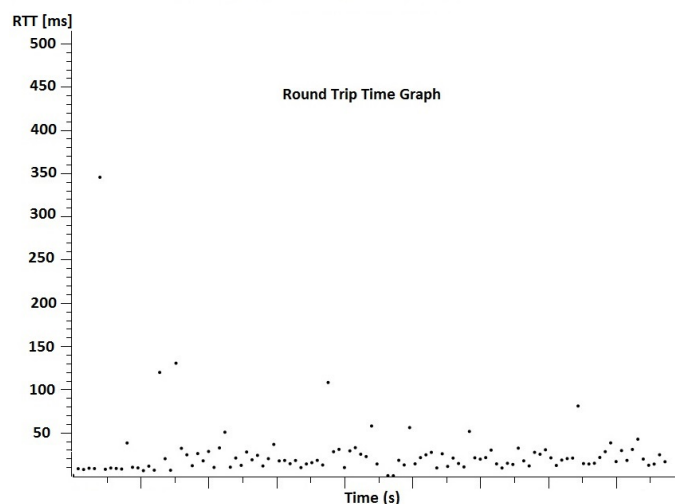
Fig. 6: Time Delay Between Smart Device 1 and Smart Device 2
