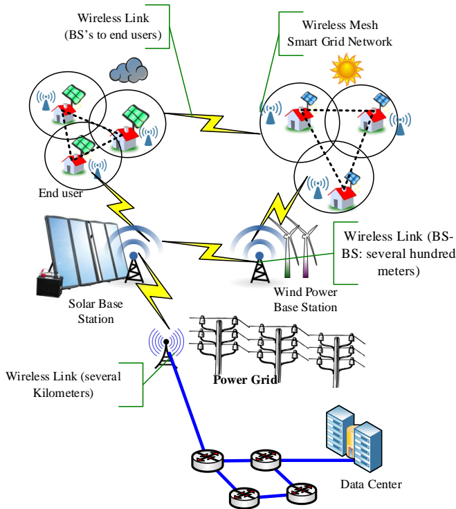
Fig. 1: Wireless mesh smart grid network exploiting green energy harvesting BS's for providing sustainable communication service by expanding communication coverage in rural areas
