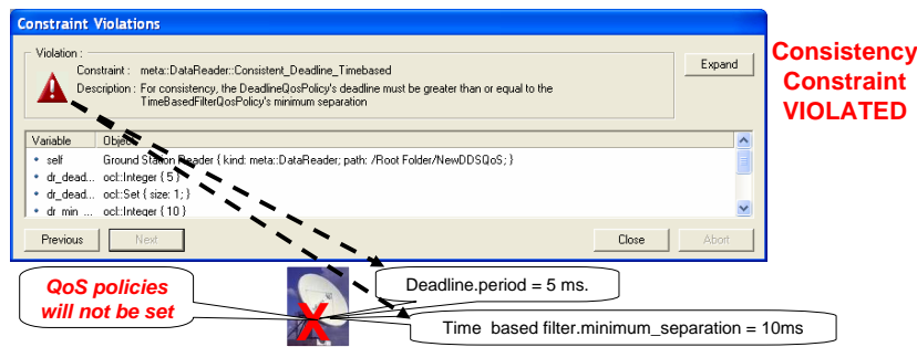
Fig. 9. Example of DQML QoS Policy Consistency Constraint Checking
