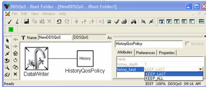
Fig. 7. Example of DQML QoS Policy Variability Management
