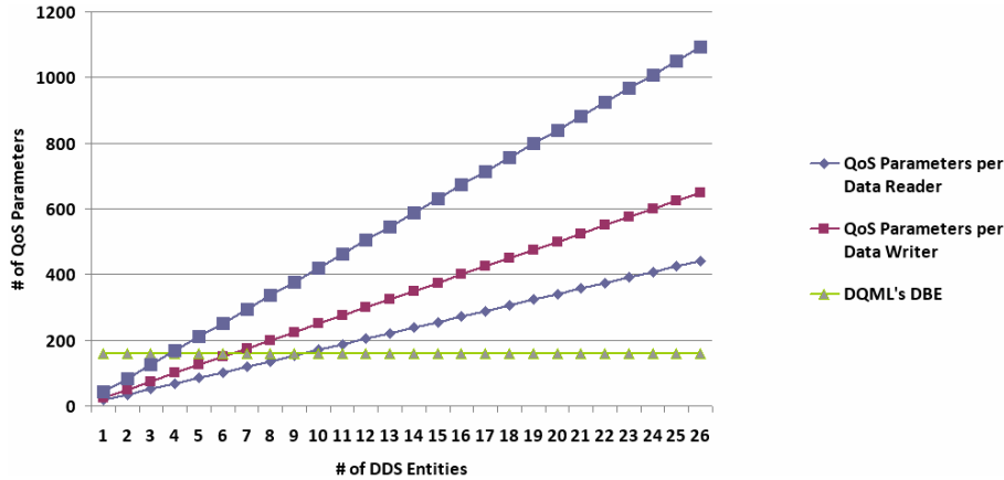
Fig. 11. Metrics for Manual Configuration vs. DQML's Interpreter
