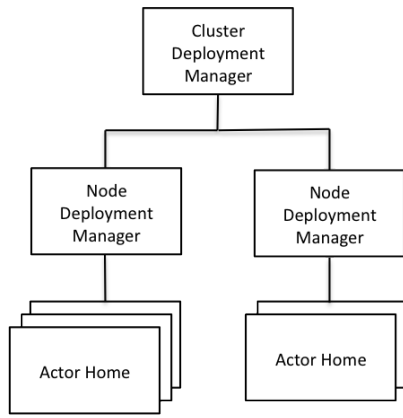
Fig. 1. Simplified F6 D&C Architecture
