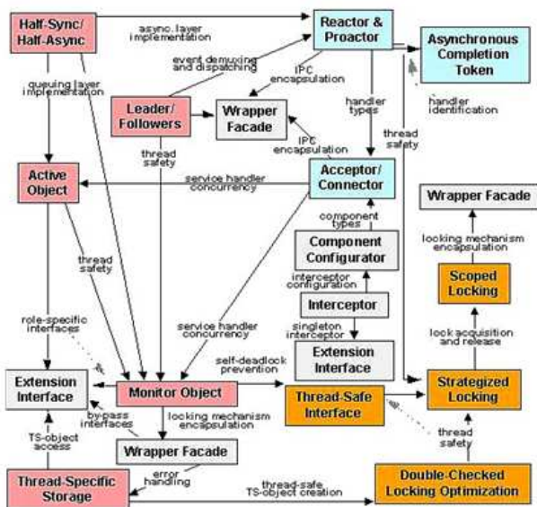
Figure 2. Middleware Patterns and Pattern Languages
