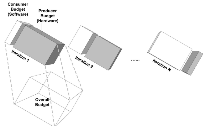
Fig. 7. Iteratively Allocating Budget to the Consumer Knapsack
