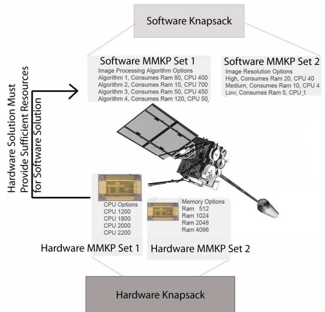
Fig. 1. Software/Hardware Design Variability in a Satellite
