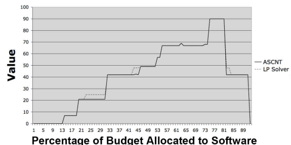
Fig. 13. Solution Value vs. Budget Allocation
