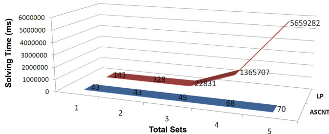
Fig. 11. Solving Time for ASCENT vs. CLP
