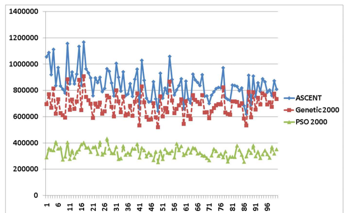
Fig. 10. Solution Score for 100 Randomly Generated Problems
