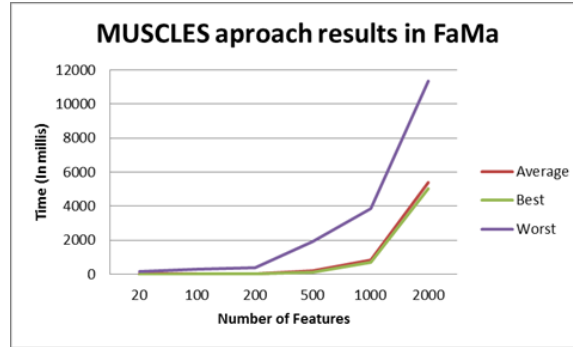
Figure 10: Automated Configuration Time for Feature Model Drift Problems
