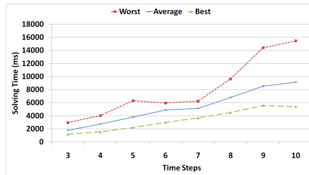
Figure 9: Automated Configuration Time for Varying Numbers of Time Steps
