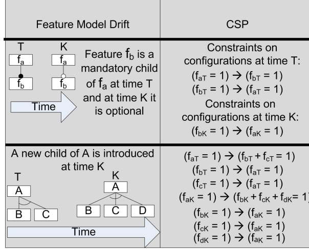
Figure 7: A CSP Model of Feature Model Drift
