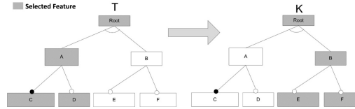
Figure 8: Changing Between Two XOR Subtrees
