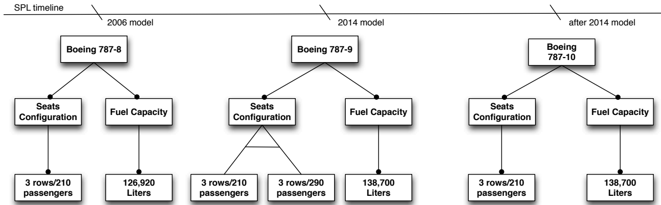
Figure 6: Boeing 787 Feature Model Drift
