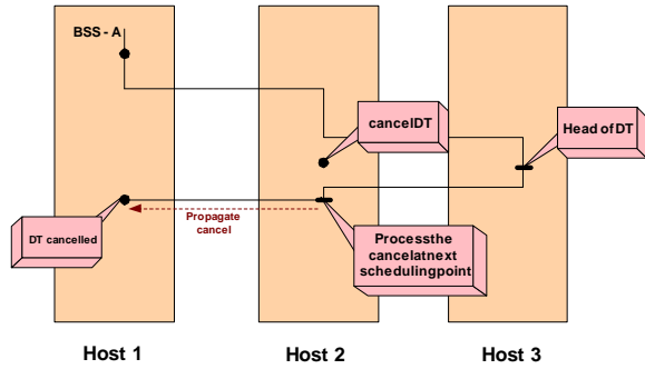
Figure 6: Distributable Thread Cancellation
