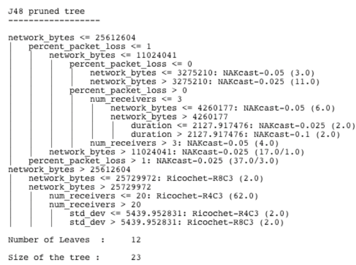
Figure 3: Initial Decision Tree
