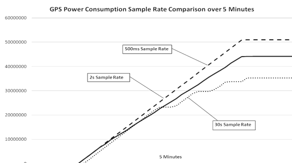
Figure 9: GPS Sample Rate Comparison
