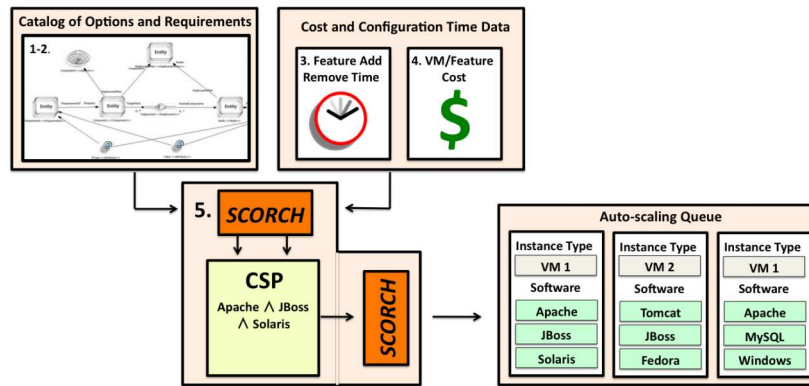
Figure 2: SCORCH Model-Driven Process
